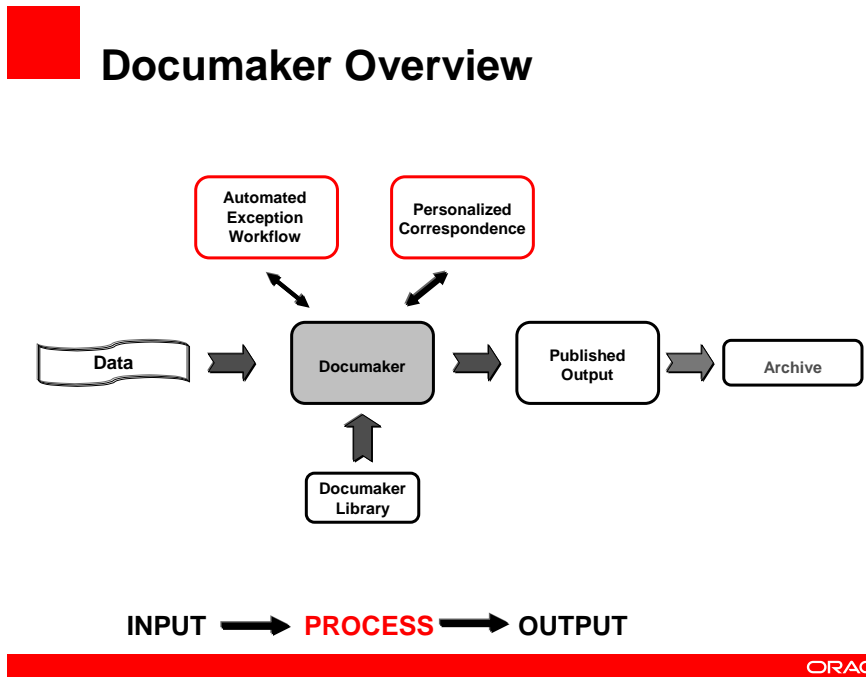
Figure 3: Documaker Overview
